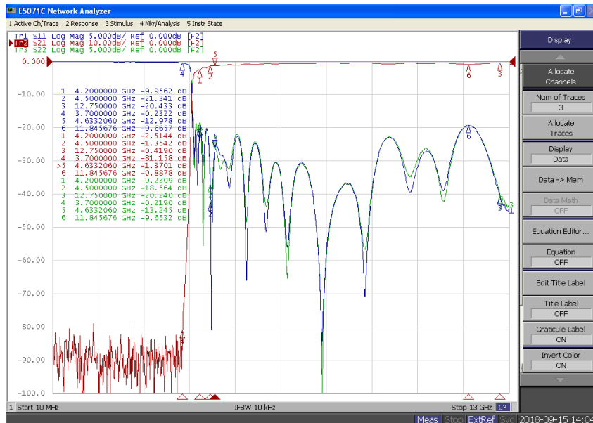
< Insertion Loss / Return Loss measurement >
